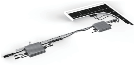
300/500G (1MPPT) 600/800/1000G3 (2MPPT) connect in parallel
